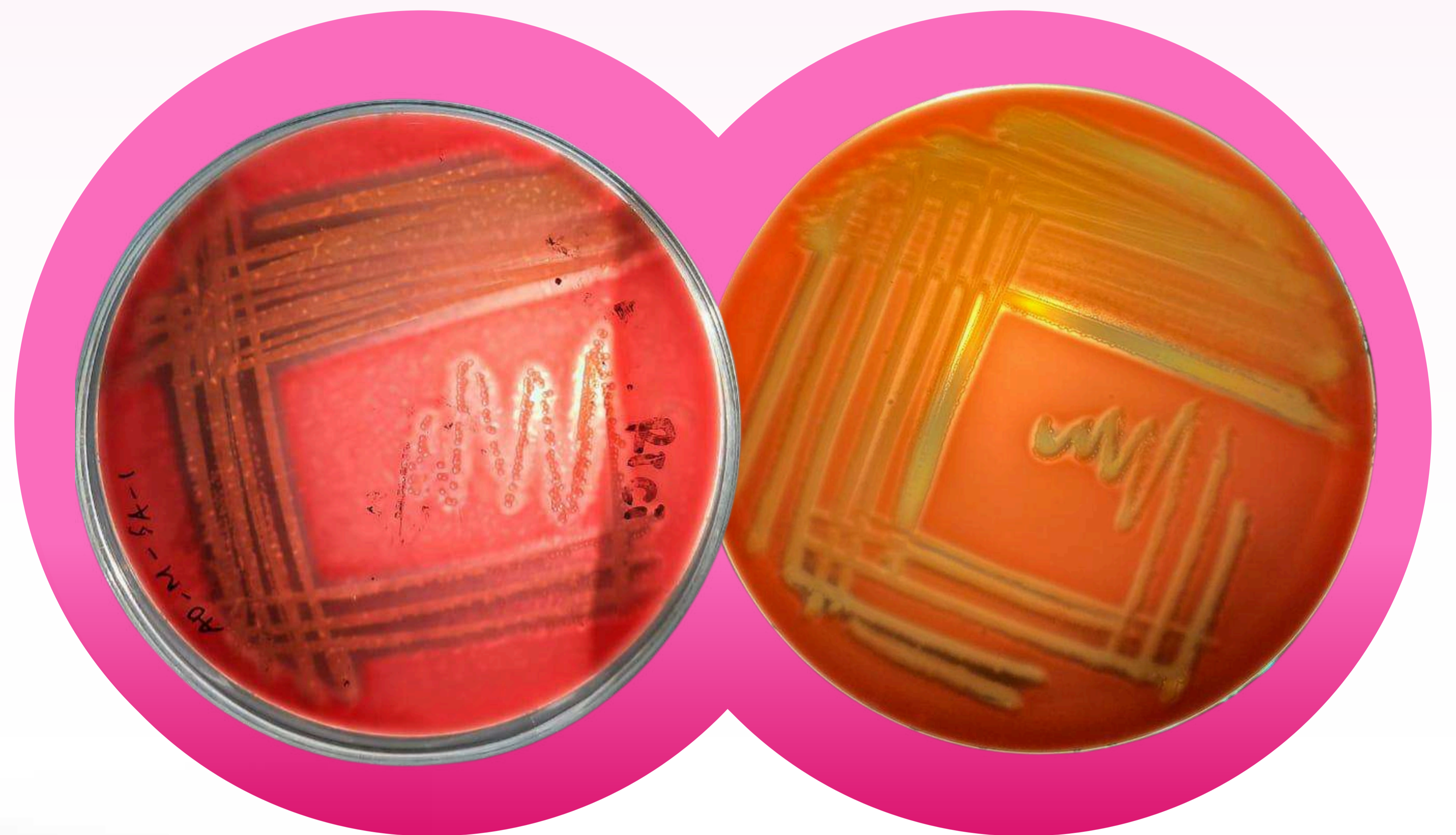
Blood Agar plate CTI (Bakteri Staphylococcus aureus ) kiri
